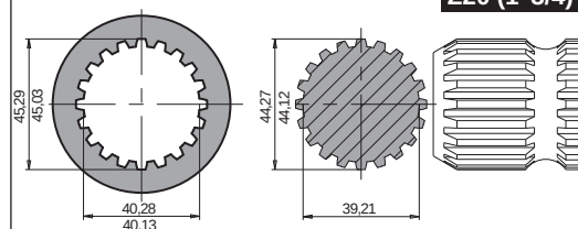
Z20 (1"3/4)
